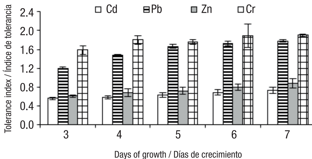
Figure 3. Tolerance index of Aspergillus niger in the presence of 10 mM of \text{CdCl}_2 , (\text{CH}_3\text{COO})_2\text{Pb}\cdot 3\text{H}_2\text{O} and \text{ZnSO}_4\cdot 7\text{H}_2\text{O} , \text{K}_2\text{Cr}_2\text{O}_7 as a source of the metals Cd, Pb, Zn and Cr, respectively. The standard deviation of the mean is shown on the bars.
